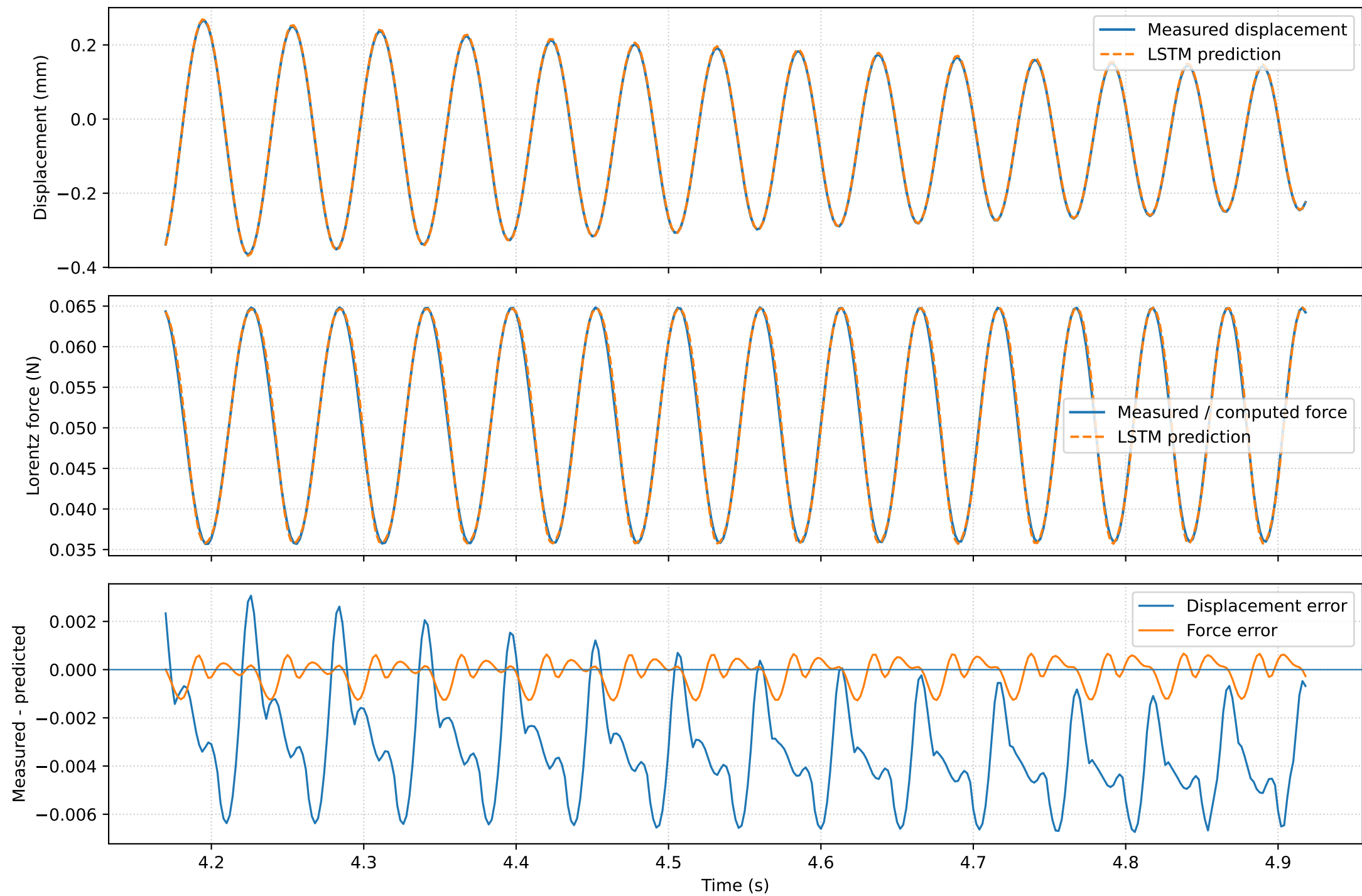
Zoomed LSTM tracking: Chirp_2 | center = 4.544 s | window = 0.750 s
